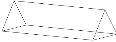
Figure 1: Attaching a 1-handle tightly
