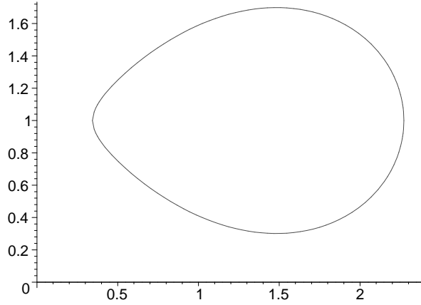
Figure 5: Profile curve of a W -surface with \kappa = \cosh \lambda + \lambda for c_0 = 1.177 .
