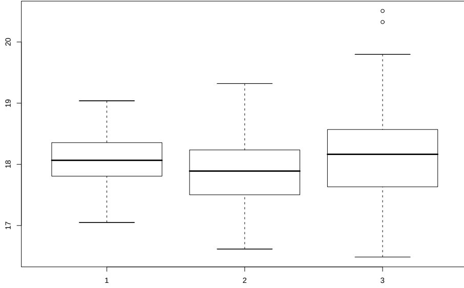
Figure 3: Results of the three different estimates in case of a jump diffusion model. Estimate 1 is the regression-based Monte Carlo estimate from Kohler (2008) based on the true jump diffusion model, for estimate 2 a Black-Scholes model is adapted to this true model, and estimate 3 is the new estimate proposed in this paper.
