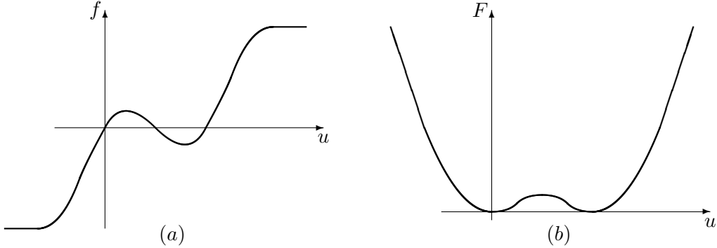
Figure 1: Example of a function f fulfilling Assumption 3.1, (a), and its associated double-well function F , (b).
